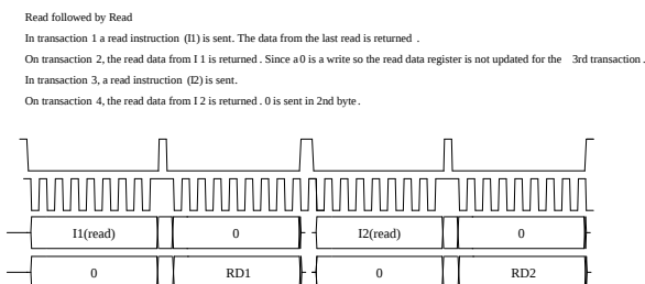
Figure 35. HPS SPI Read Timing (Read/Read)
